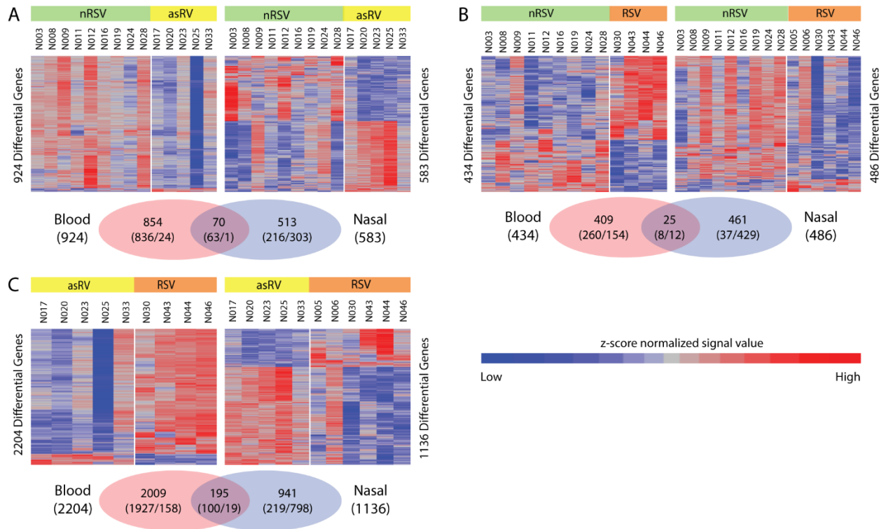
Figure S4. Heatmap and Venn diagrams for 2-way comparisons between each pair of the 3 viral groups in both blood and nasal samples: non-RSV vs. asRV (A), non-RSV vs. RSV (B), and asRV vs. RSV (C). Within the Venn diagram, numbers in parenthesis indicate up/down-regulated genes.
