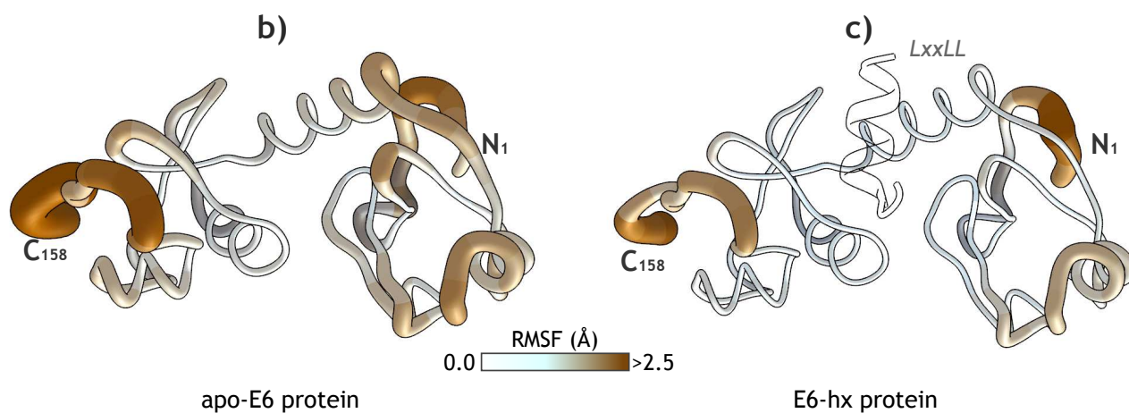
Figure S5: RMSF values of the E6 protein in the apo-E6 and E6-hx systems. a) RMSF values of each residue of the E6 protein (apo-E6 = red, E6-hx = blue). Bold lines correspond to the average RMSF values of the three assays of each system, and semitransparent ribbons display the standard deviations. The gray columns in the background indicate the position of pocket residues. b) and c) Structural representation of the E6 backbone showing, in a color range (white to brown), the most flexible regions of the protein according to the RMSF value of each residue in each system: apo-E6 and E6-hx.
