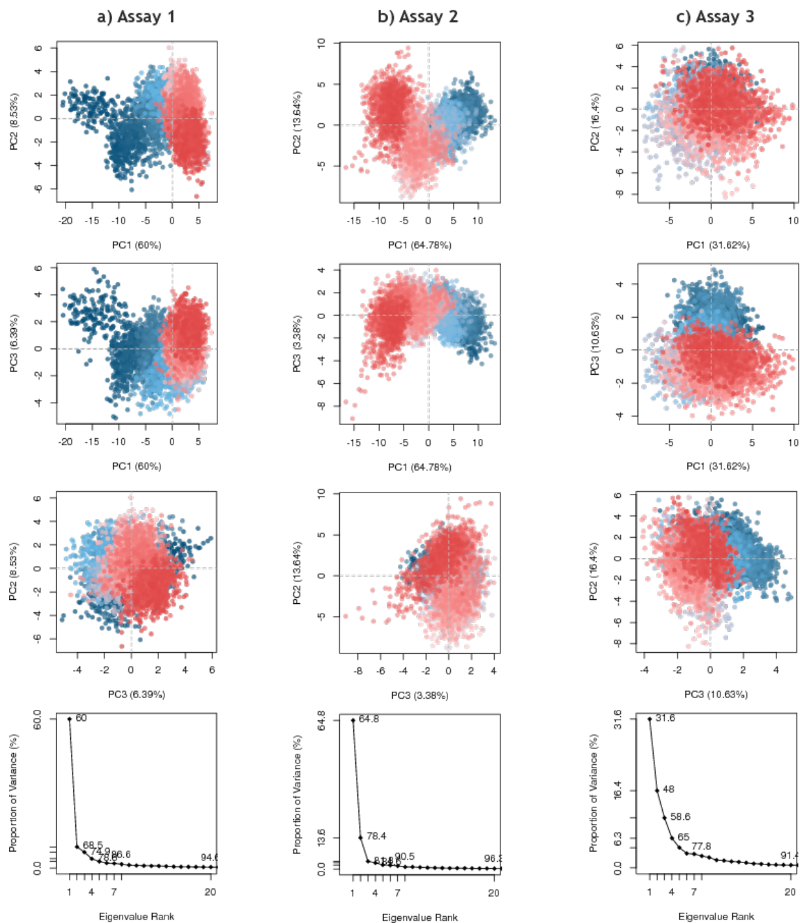
Figure S6: Principal Component Analysis of the three apo-E6 trajectories. Scatter plots and scree plots of the first three PCs (red: 0 ns to blue: 100 ns) from Assay 1 (a), Assay 2 (b) and Assay 3 (c) of apo-E6 system.
