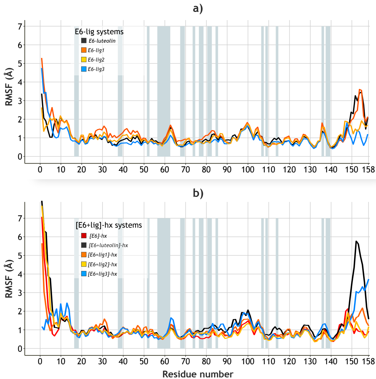
Figure S11: RMSF values of the E6 protein in the E6-lig and [E6+lig]-hx systems. a) E6-lig systems, b) [E6+lig]-hx systems. The gray columns in the background indicate the position of pocket residues.
