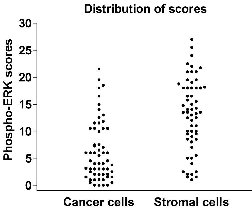
Supplementary Figure 1: Scattergram illustrating the distribution of scores for nuclei in cancer cells and stromal cells.
