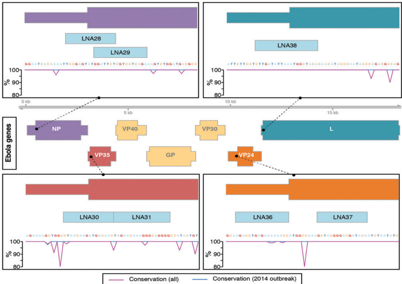
SUPPLEMENTARY FIG. S1. Binding sites of LNA ASO mixmers targeting Ebola transcripts. Diagram showing the coding regions of the Ebola virus. A detailed view of the regions surrounding transcriptional start sites of targeted virus transcripts and binding sites of the LNA ASOs are shown in the panels . LNA, locked nucleic acid; ASO, antisense oligonucleotide.
