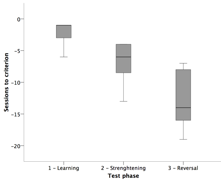
S2 Fig. Number of test sessions to criterion in the 3 phases of the Reversal Learning task. Fewer (12-trial) sessions indicate better performance, hence the negative prefix on the y-axis. Phase 1 - learning of the initial association between a pattern and a reward. Phase 2 - strengthening of the learned association. Phase 3 - reversal of the learned association.
