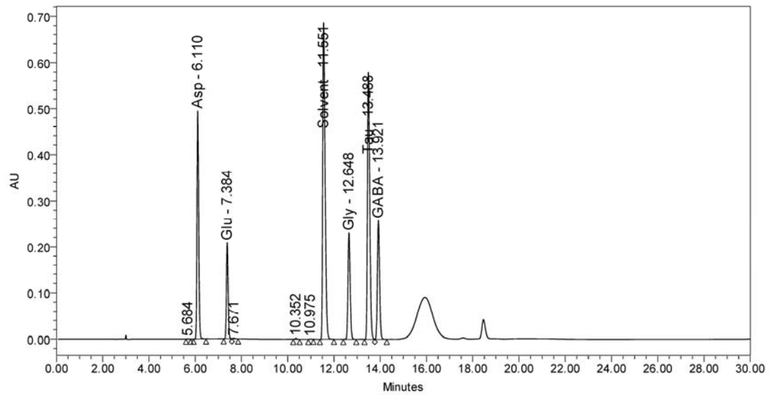
Fig. S1. HPLC chromatogram of standard mixed solution of five amino-acids.
