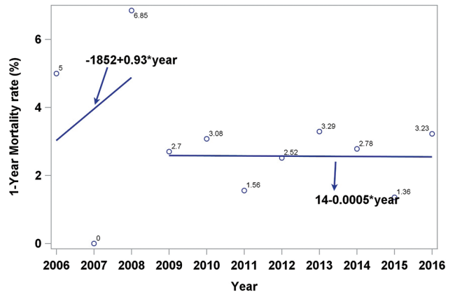
SUPPLEMENTAL FIGURE S2. Piecewise regression: a time trend of 1-year all-cause mortality.
