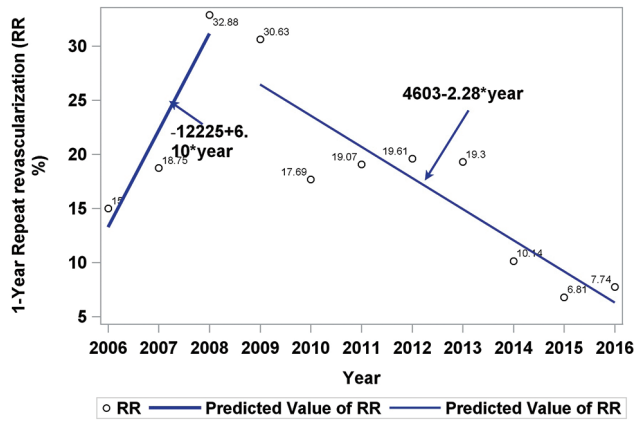
SUPPLEMENTAL FIGURE S1. Piecewise regression: a time trend of 1-year repeat revascularization (RR).
