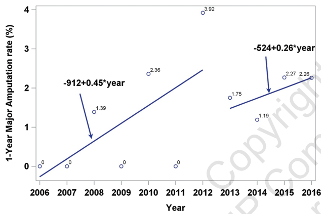
SUPPLEMENTAL FIGURE S3. Piecewise regression: a time trend of 1-year major amputation.
