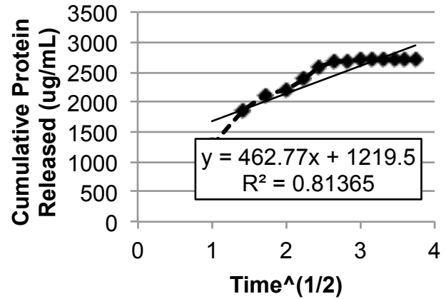
E Higuchi Release Model
