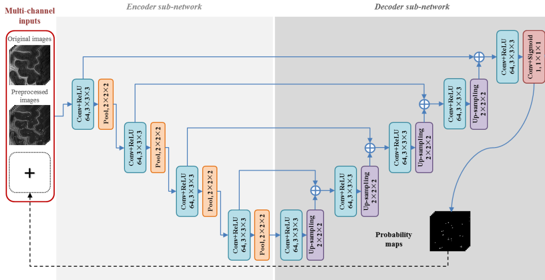
Figure S1: The network architecture of M^2EDN-S , i.e., a single-scale variant of the proposed M^2EDN . That is, no multi-scale feature learning is included in M^2EDN-S .
