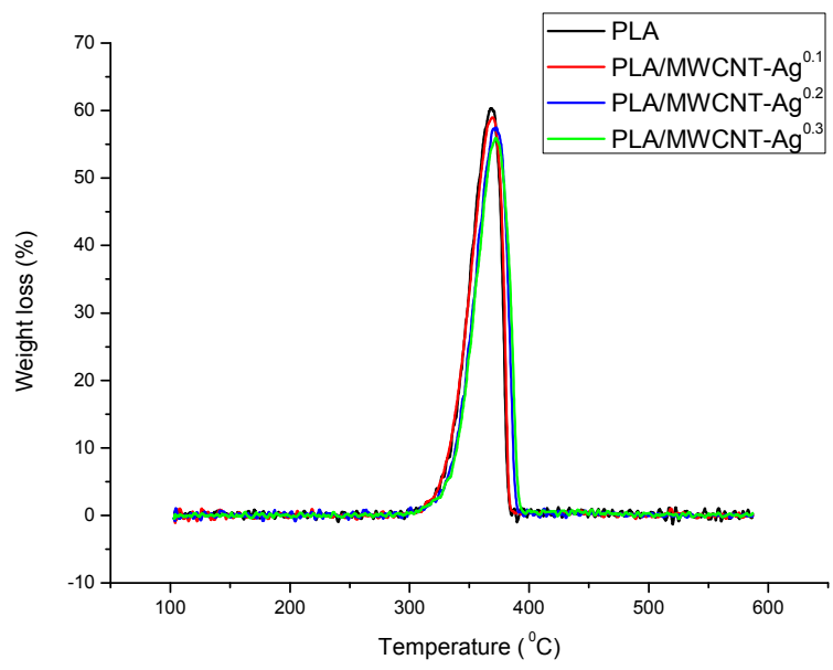
Figure S3. DTG curves of PLA and PLA/MWCNT-Ag nanocomposites.
