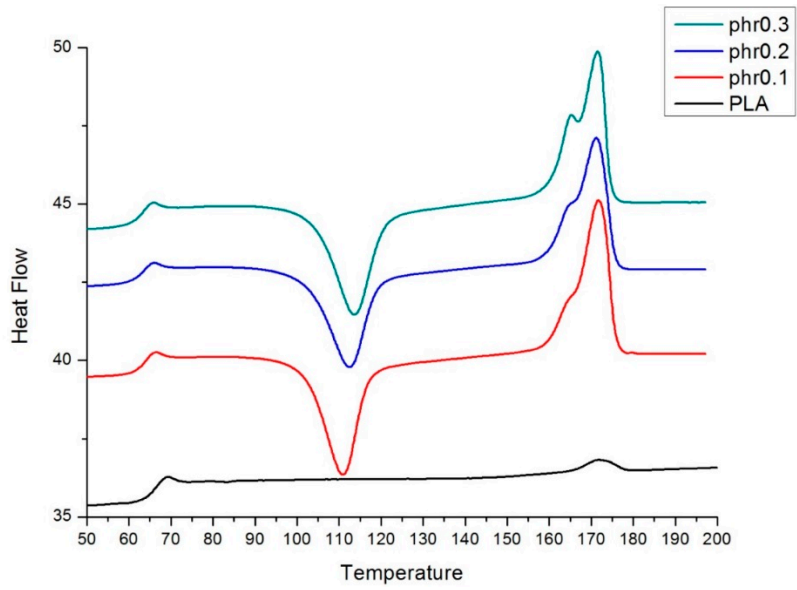
Figure S4. DSC curves of PLA and PLA/MWCNT-Ag nanocomposites.
