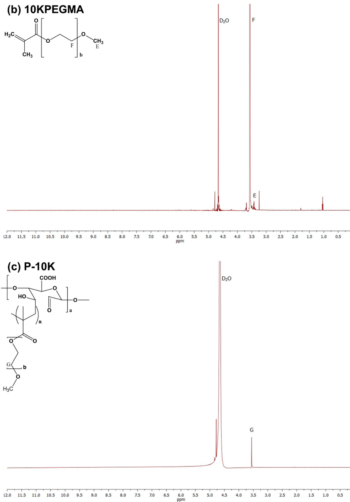
Figure S1. 500 ^1\text{H} NMR spectra of the precursors (pectin and 10KPEGMA) and copolymer P-10K.
