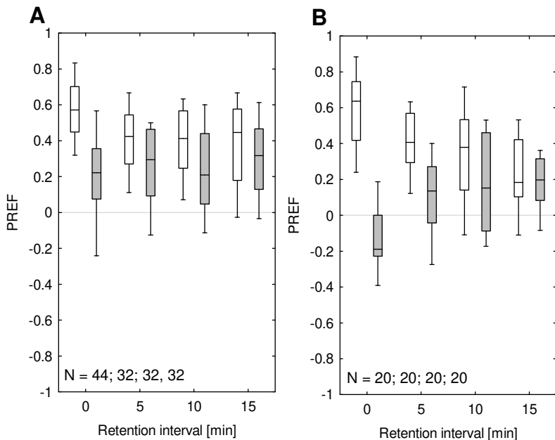
Figure S7: Preference scores underlying the performance indices from Figure 7. Documentation of preference scores (PREF) after paired (open boxes) and unpaired (boxes with grey fill) training for the indicated retention intervals for animals trained (A) once, or (B) three times. Data are displayed as box plots, with the median as the middle line, the box boundaries as 25 and 75 % quantiles, and the whiskers as 10 and 90 % quantiles. Sample sizes are indicated within the figure.
