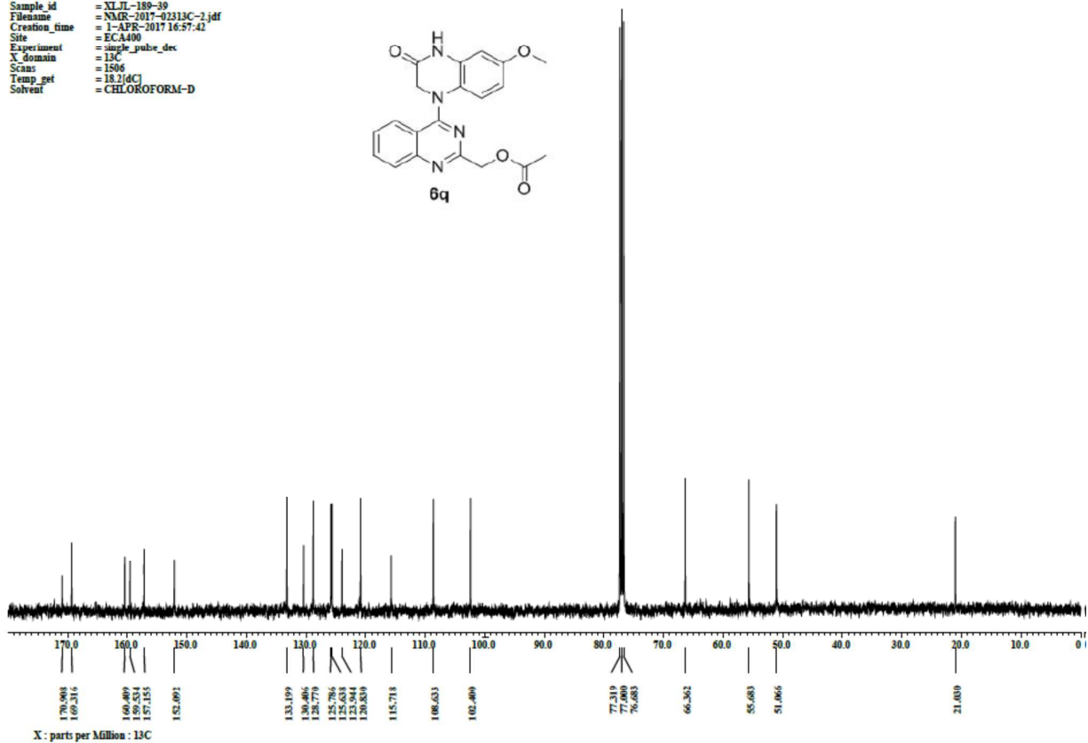
Figure S4. ^{13}\text{C} NMR spectra of 6q
