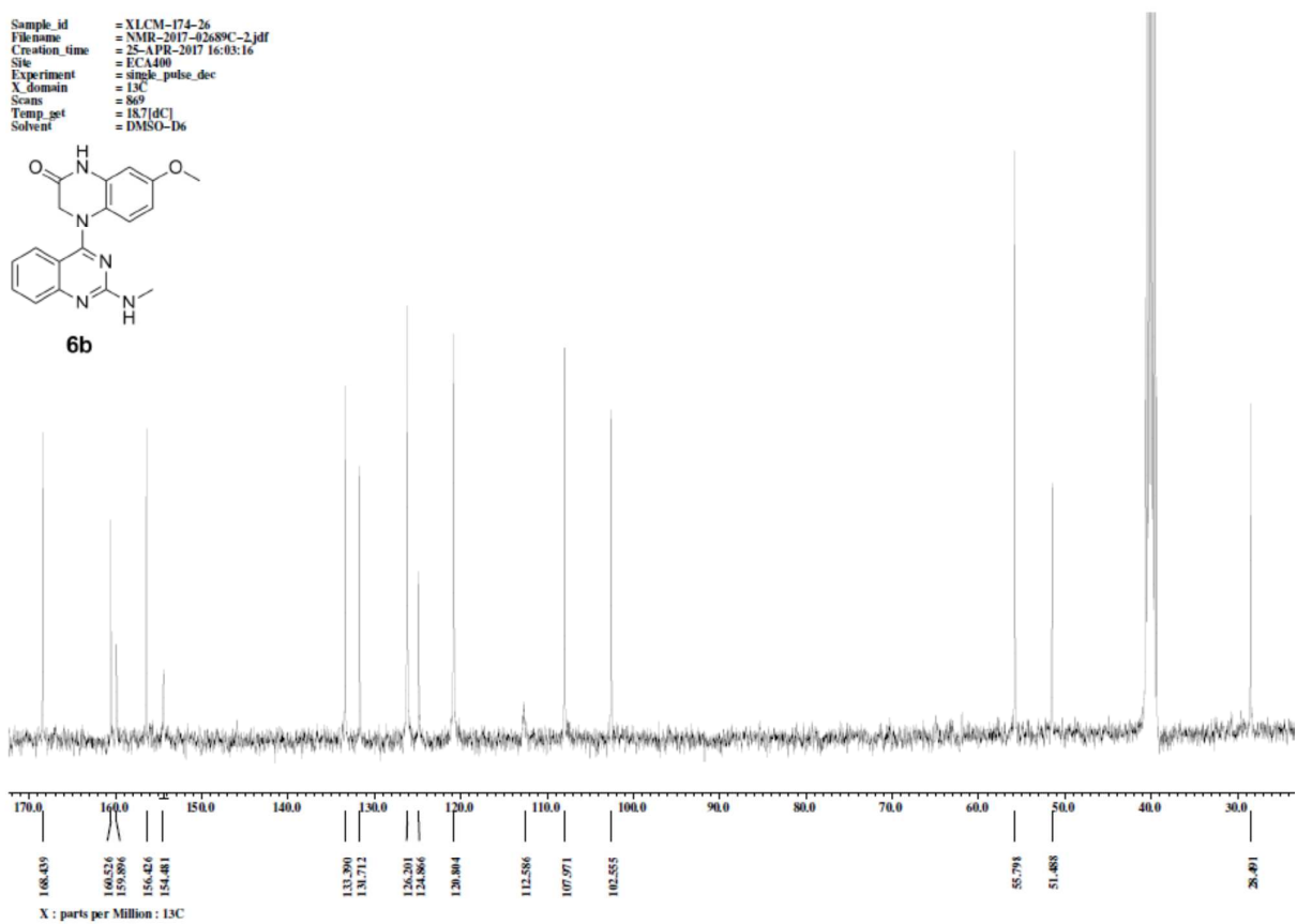
Figure S2. ^{13}\text{C} NMR spectra of 6b
