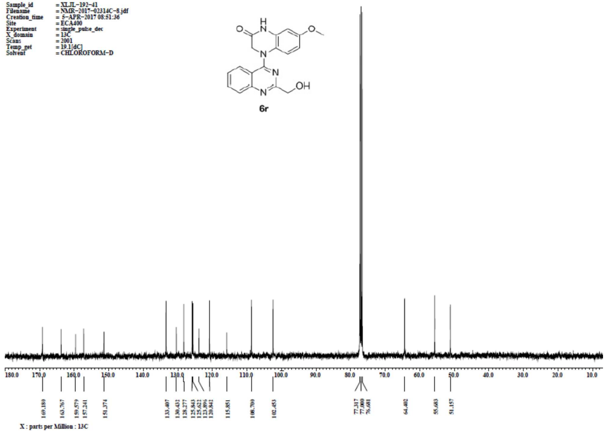
Figure S5. ^{13}\text{C} NMR spectra of 6r
