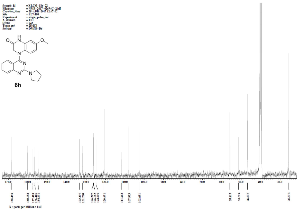
Figure S3. ^{13}\text{C} NMR spectra of 6h
