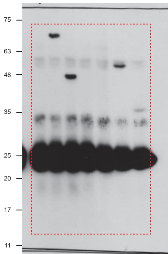
IP anti-Flag
