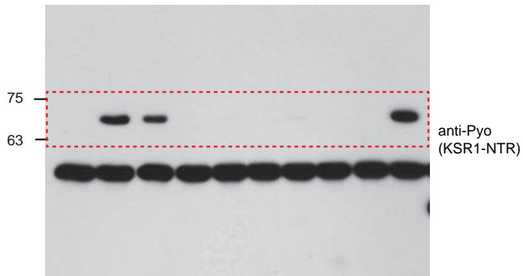
IP anti-Flag
