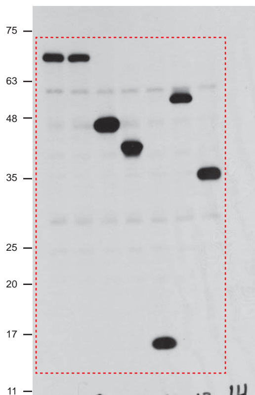
Lysates
