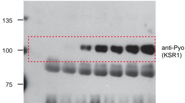
IP anti-Flag
