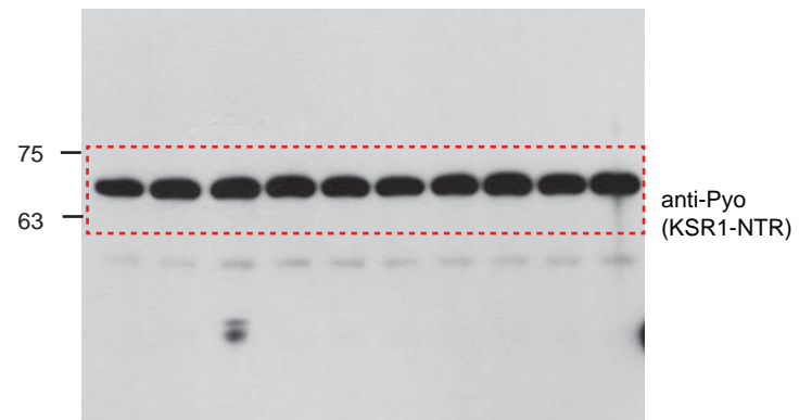
Lysates
