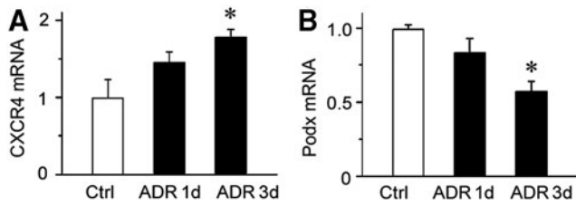
SUPPLEMENTARY FIG. S1. The mRNA expressions of CXCR4 and podocalyxin are changed after ADR injection. Graphical representations of the relative abundances of CXCR4 (A) and podocalyxin (Podx) (B) mRNA in different groups as indicated. * p < 0.05 versus normal controls ( n = 5-6 ). ADR, adriamycin nephropathy; CXCR4, C-X-C chemokine receptor type 4; mRNA, messenger RNA.
