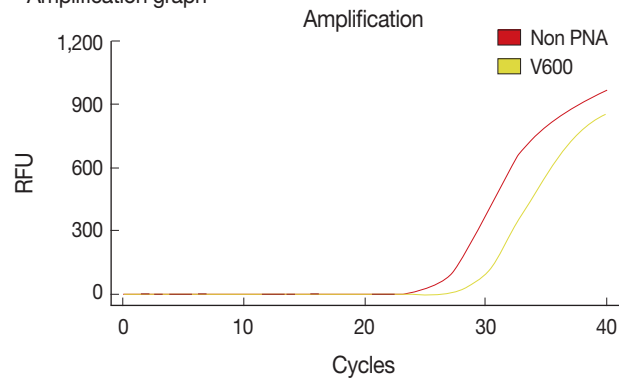
Supplementary Fig. S1. BRAF V600E mutation is confirmed in case 1 by real-time polymerase chain reaction using a peptide nucleic acid (PNA) clamping method.
