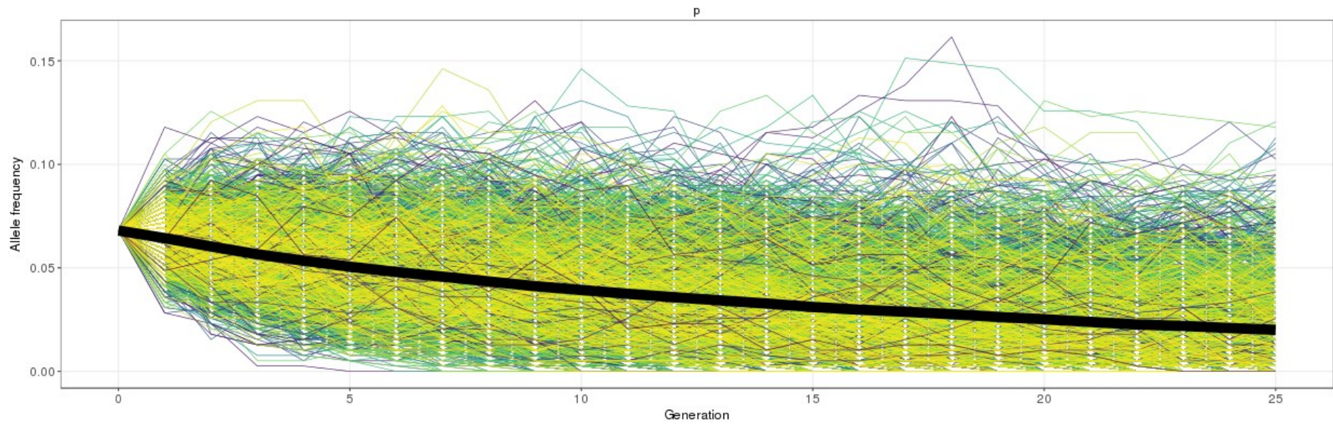
Figure S1: Genetic drift simulation for a lethal recessive with an allele frequency of 6.7% (13.4% carrier frequency) over 25 generations. Plot shows frequency after 25 generations for 1000 simulations. The allele is lost in approximately 30% of the simulations. In 7.5% of the simulations the frequency after 25 generations is equal or greater than the start frequency.
