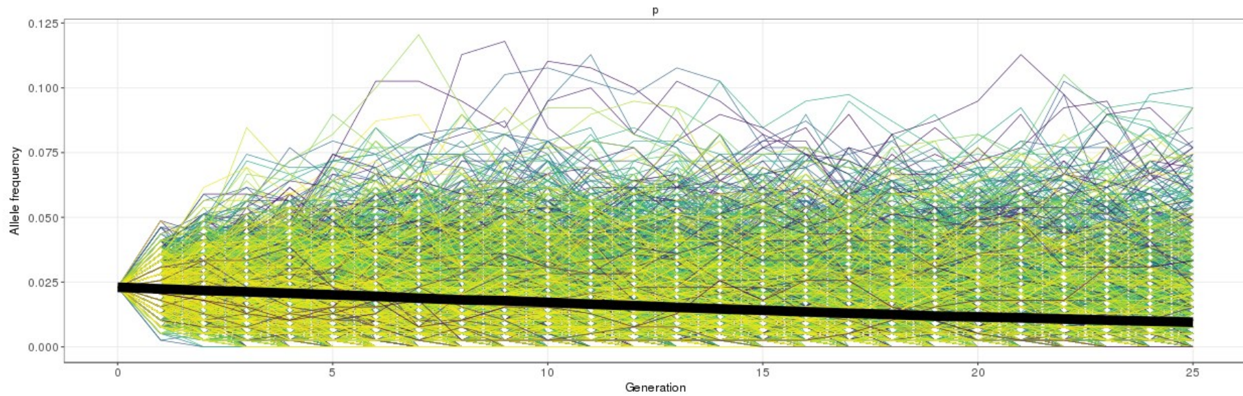
Figure S2: Genetic drift simulation for a lethal allele with 2.3% allele frequency (carrier frequency: 4.6%) over 25 generations. Plot shows frequency after 25 generations for 1000 simulations. The allele is lost in approximately 62% of the simulations, while in 25% of the simulations the frequency after 25 generations is equal or greater than the start frequency.
