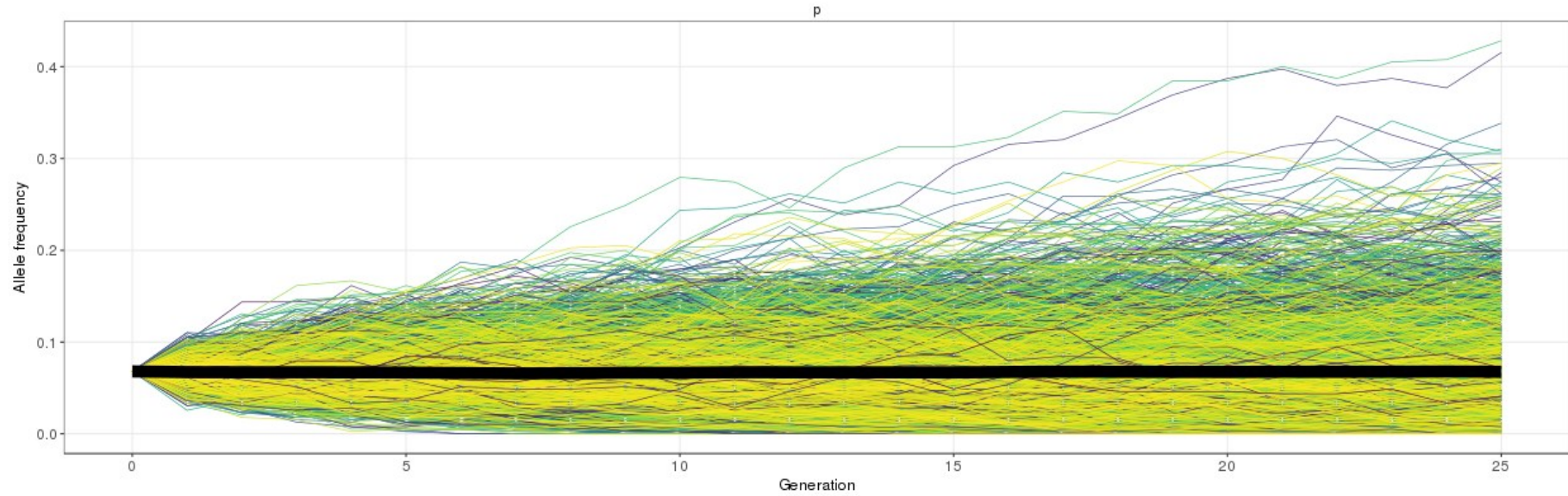
Figure S3: Genetic drift simulation for a neutral allele with 6.7% allele frequency (13.4% carrier frequency) over 25 generations. Plot shows frequency after 25 generations for 1000 simulations. The allele is lost in approximately 14% of the simulations, while in 49% of the simulations the frequency after 25 generations is equal or greater than the start frequency.
