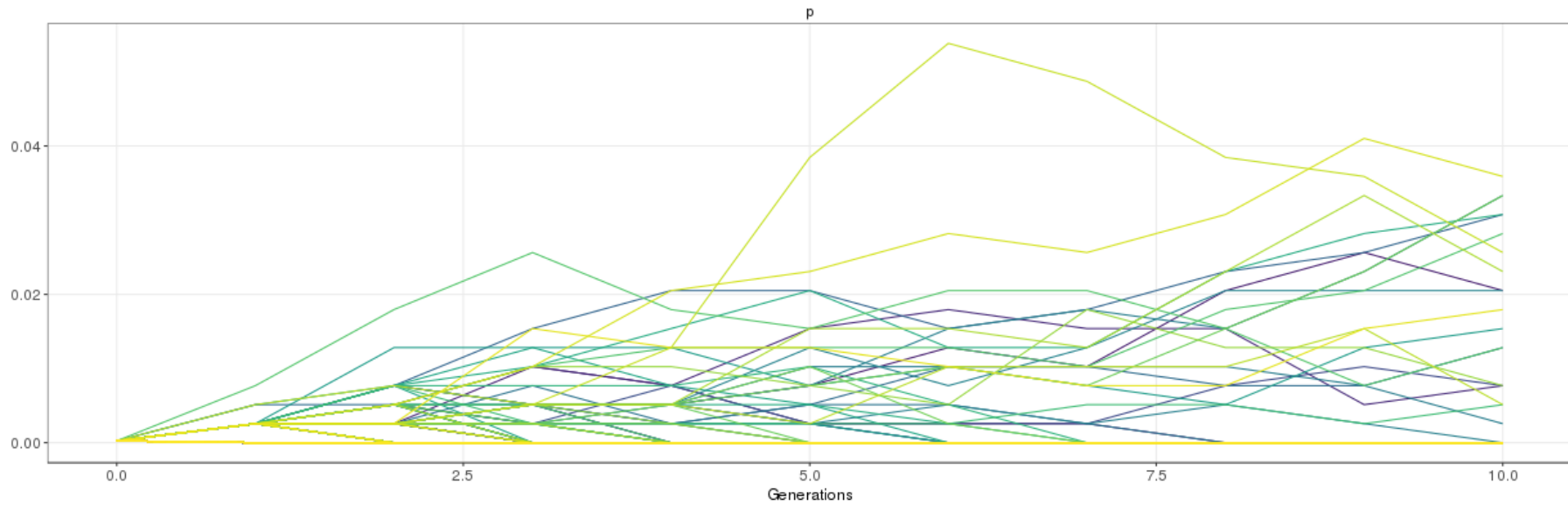
Figure S4: Genetic drift simulation for a de novo mutation with start frequency of 0.024% over 10 generations. Plot shows that in 20 out of 1000 simulations (2%) the de novo mutation is still segregating in the population after 10 generations.
