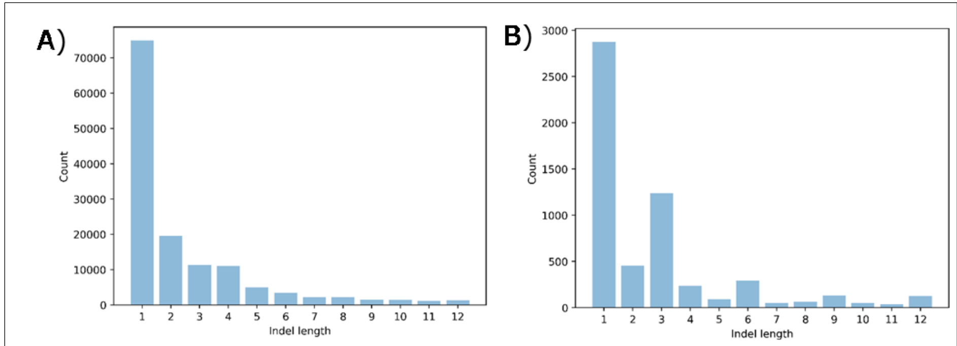
Figure S7: Enrichment of inframe indels in coding regions. A) Indel length distribution for non-coding regions. B) Indel length distributions for coding regions. Figure shows an enrichment of inframe indels in coding regions (e.g. length 3,6,9), not shown in non-coding regions.
