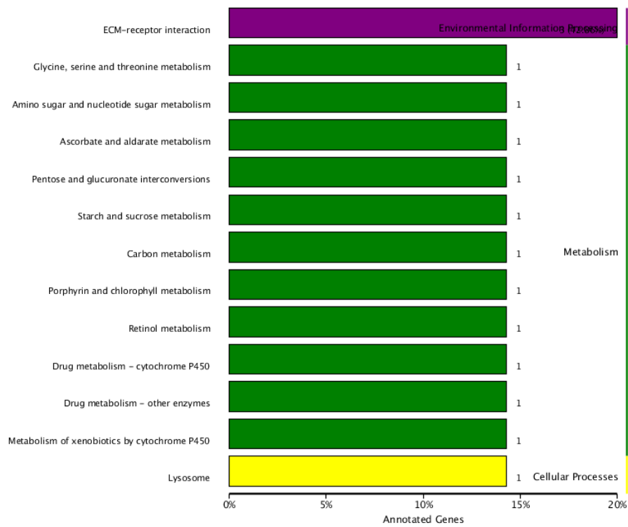
Figure S3. KEGG classification analysis for predicted differentially expressed genes (DEGs) of differentially expressed miRNAs (DEMs) in WS vs. LWS.
