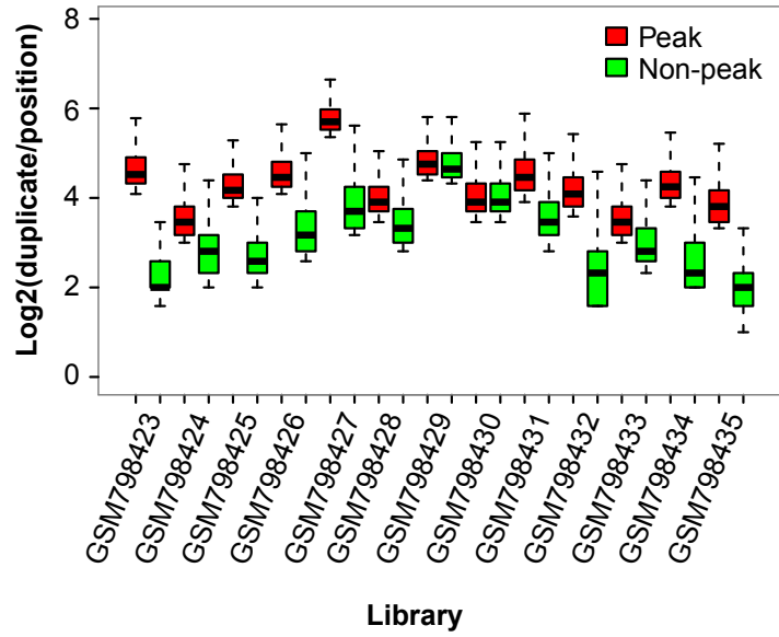
S4 Fig. Box plot of the number of duplicates per position. The top 10,000 positions with the most duplicates from both ER peaks and non-peak regions were analyzed. Non-peak regions are those not covered by peaks.
