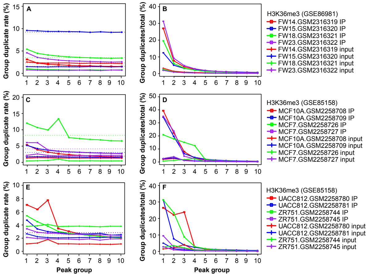
S6 Fig. Duplicate rate versus confidence level of H3K36me3 peaks. (A,C,E)
