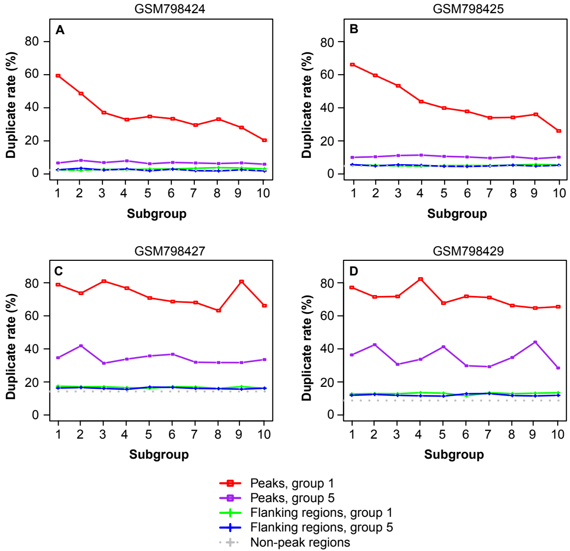
S9 Fig. Duplicate rate in ER peaks and the flanking regions. Peaks from group 1 (top 10% peaks with the lowest p values) and 5 (the fifth decile) were both split into 10 subgroups of equal size. Non-peak regions are 100 bp away from peaks. Flanking regions are peak 5' and 3' regions that are 300-bp away from the peaks and have the same size as the peaks. See S1 Table for sample information.
