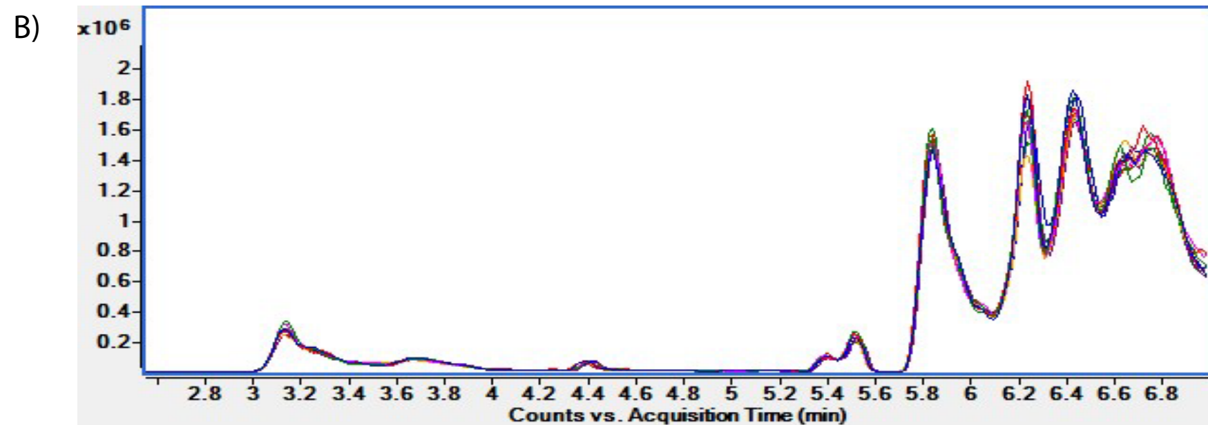
Supplementary Figure 1. Total ion chromatogram of pooled BLCA serum samples (A) ESI positive ionization mode (B) ESI negative ionization mode.
