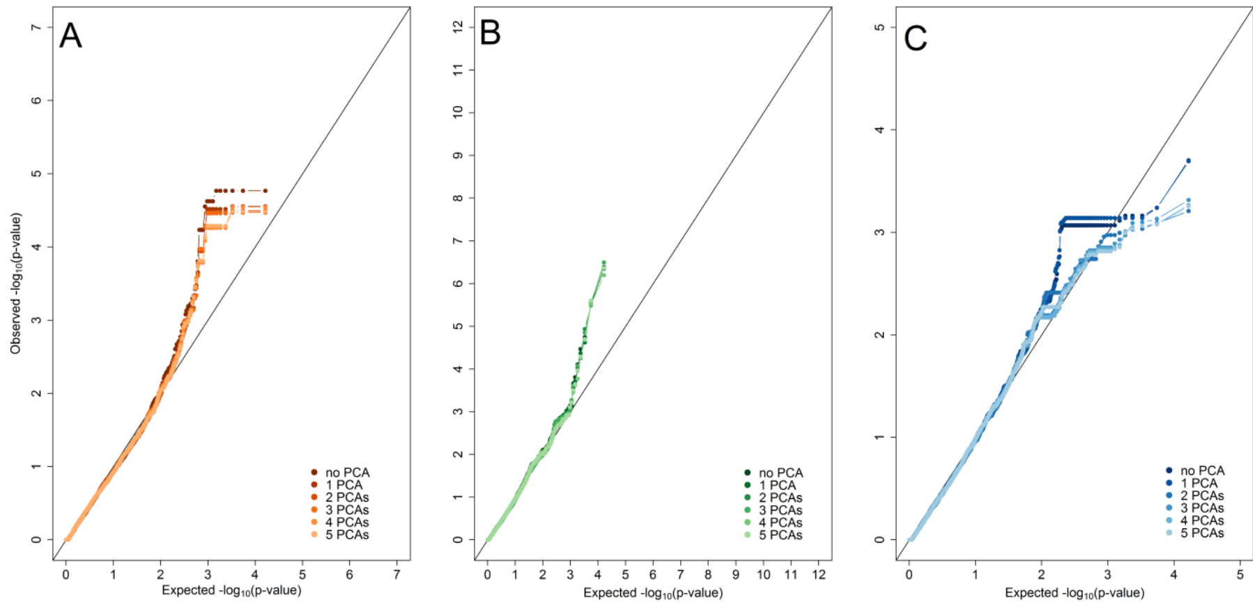
Fig. S1 Quantile-quantile plot of the expected versus observed -\log_{10}(P) values for FHB severity (A), plant height (B), and flowering date (C) modelling none or the 1-5 first principal components as fixed effect in the mixed model employed for genome-wide association mapping additional to correcting kinship by a genomic relationship matrix
