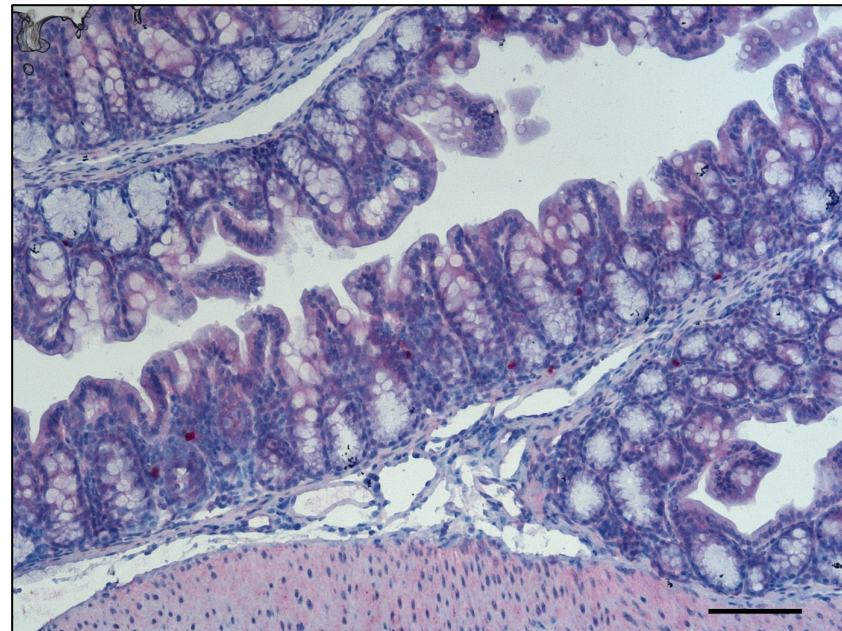
Naive
