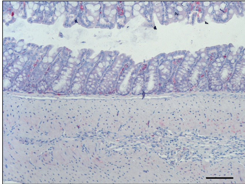
Naive
