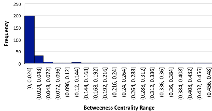
Betweenness Distribution
