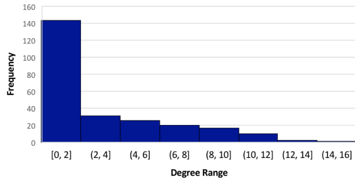
Degree Distribution
