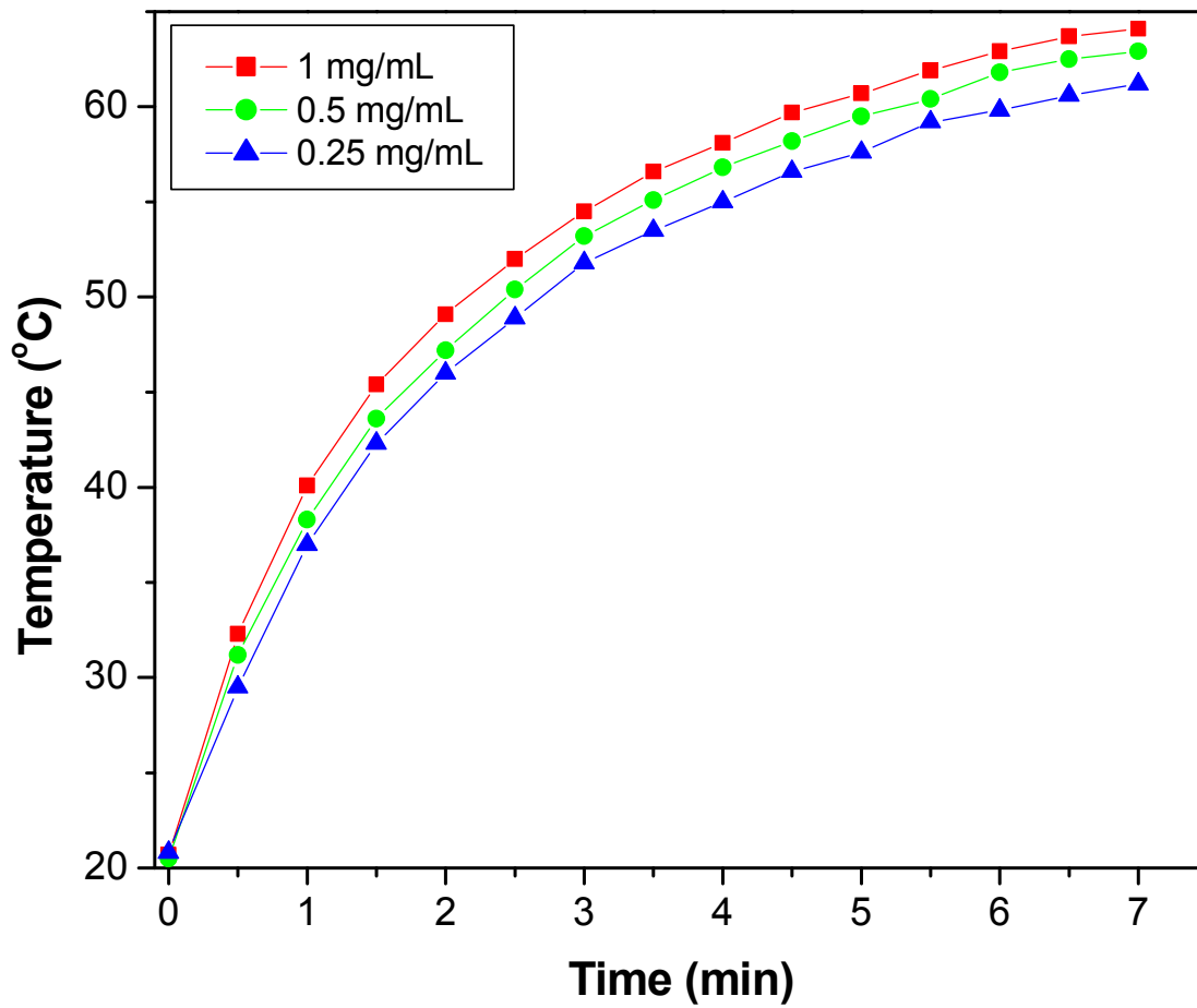
Figure S1 Photothermal effect of CNTs-PAMAM/G4-CdS at different concentrations.
