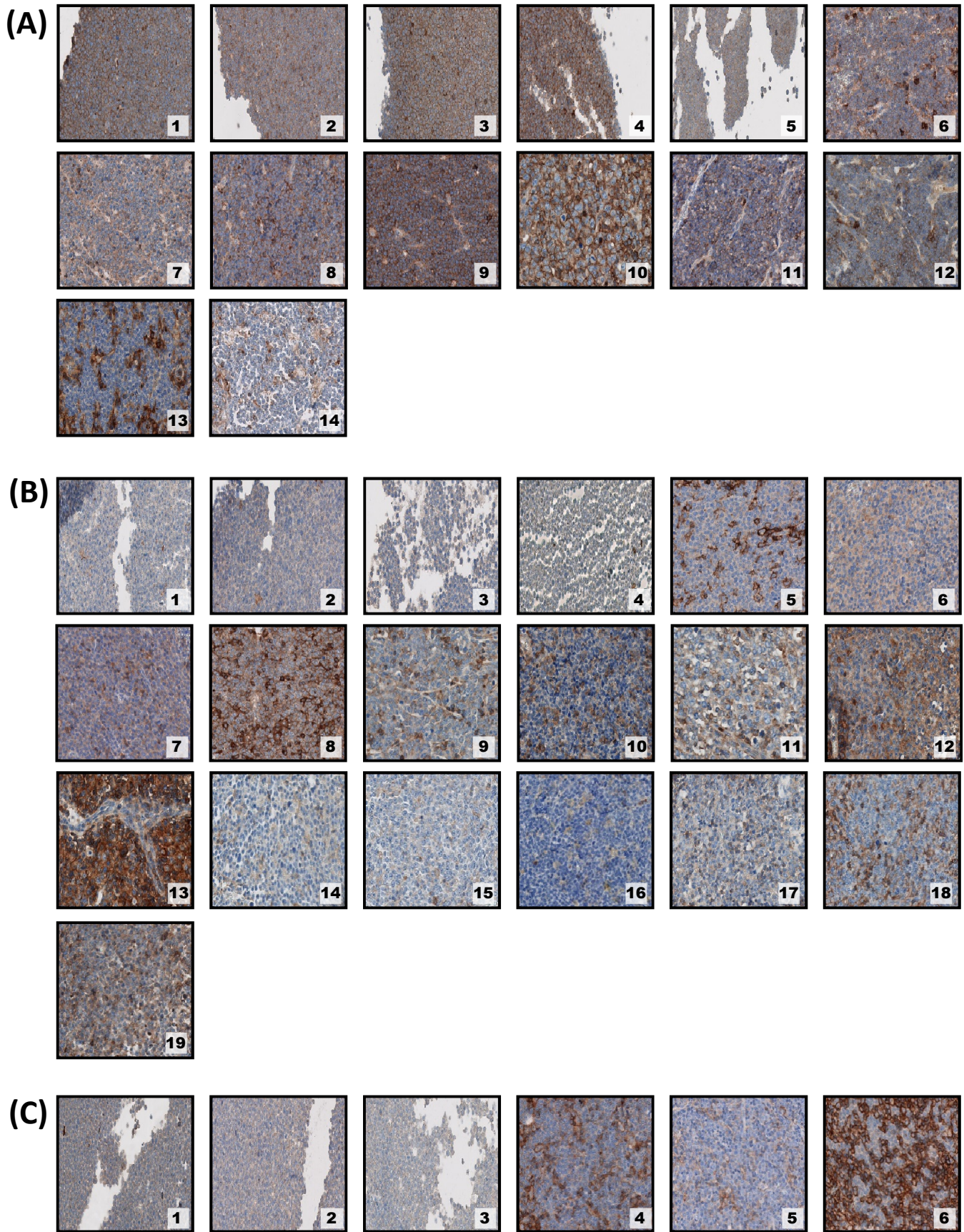
S4 Figure. ADGRE5 IHC staining of cell line and patient tissue samples. (A) Burkitt Lymphoma (BL): Cell lines (1-5: Blue-1 BL-41, BL-2, DG-75, CA-46) and primary tumor tissues (7-14) are mainly ADGRE5 positive. (B) Diffuse large B-cell lymphoma without MYC break (DLBCLneg): Cell lines (1-4: Karpas-422, U2932-R1, HT, WSU-DLCL2) and primary tumor tissues (5-19). (C) DLBCLpos: Cell lines (1-3: Carnaival, U2932-R2, SU-DHL-10) and primary tumor tissues (4-6). DLBCLpos and DLBCLneg are mainly negative for ADGRE5. Strong positive staining in some tissue sections results from macrophages or T-cells.
