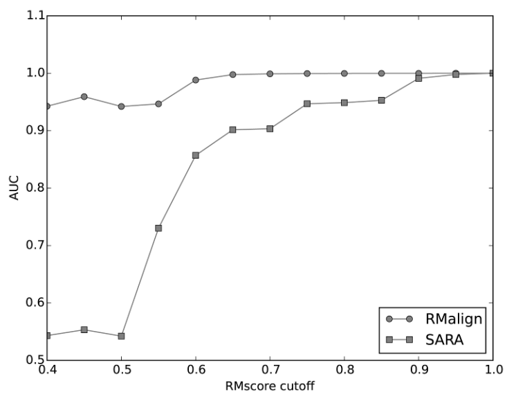
Figure S7. Benchmarking of RAlign and SARA in balance-x-FSCOR .
