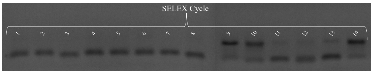
S1 Fig. Aptamer enrichment analysis by the DiVE assay. See materials and methods for further details.
