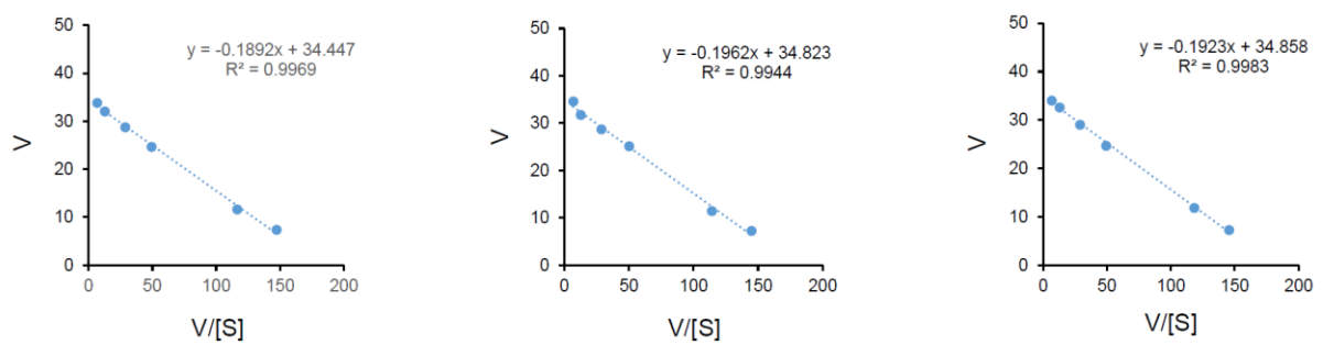
Fig S2. Kinetic parameters determined with Eadie-Hofstee plots.
