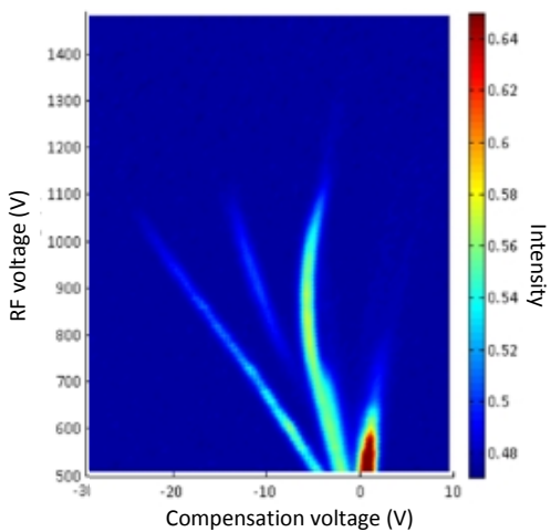
Supplementary Figure: DMS dispersion plot of 500 ppb of 2-butanone and ethyl acetate at 80°C drift tube temperature.
