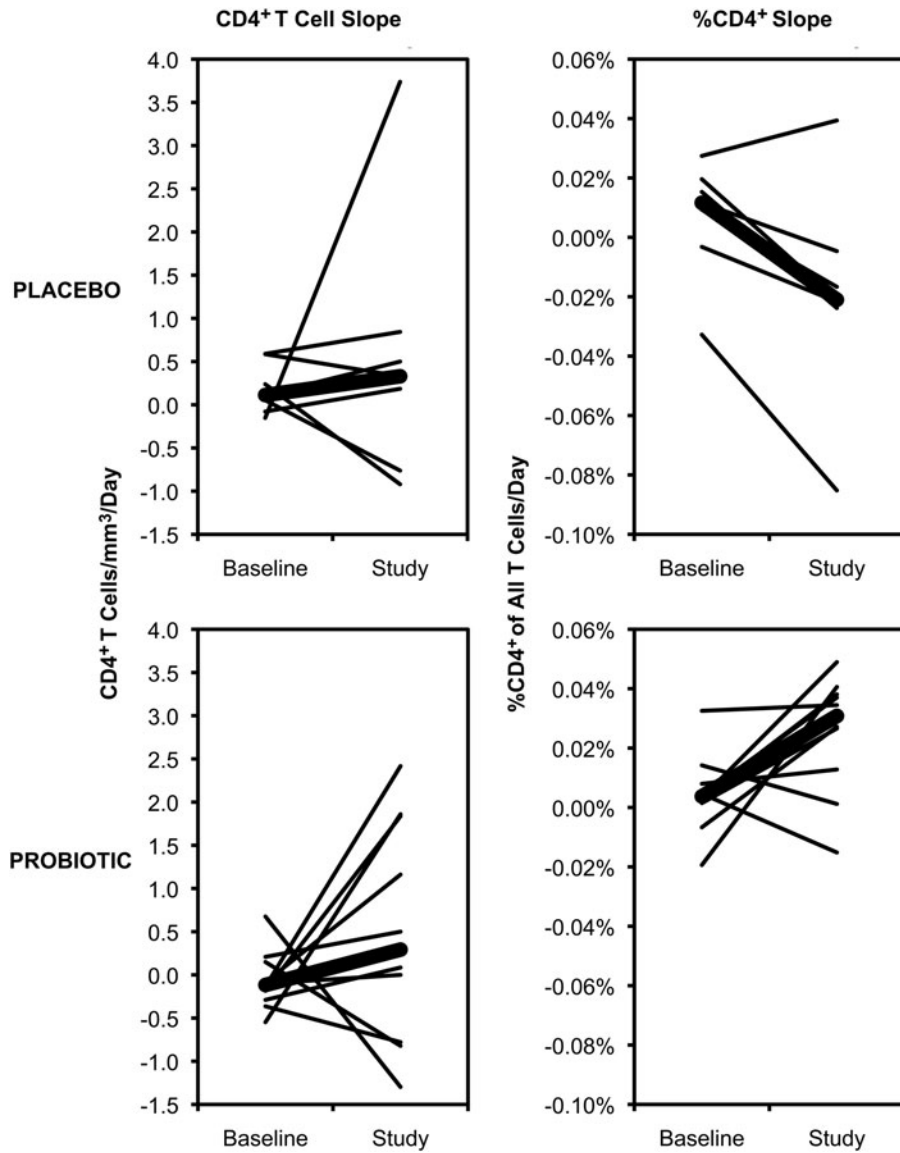
SUPPLEMENTARY FIG. S1. Slopes of blood CD4 + T cell counts and percentages during the study compared to the prior year. The slopes of blood CD4 + T cell counts and percentages ( \Delta CD4 + T cells/mm 3 /day and \Delta % CD4 + T cells/day) at baseline (determined by three measurements in the prior year and the start of placebo or probiotic administration) and during the study (determined by measurements from the start to the end of placebo or probiotic administration) are plotted for placebo and probiotic groups. Each thin line represents an individual, and the thick lines indicate medians for each group.
