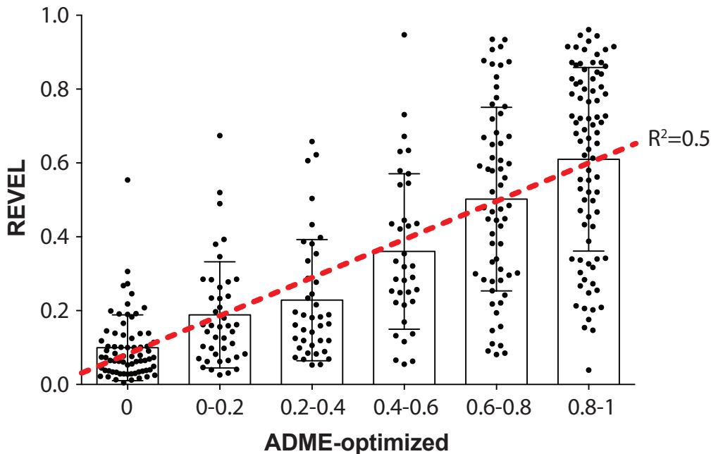
Supplementary Figure 3: Scores derived by the ADME-optimized prediction model correlate with REVEL scores. Note that while the scores between the models overall correlate, predictions for individual variants can diverge substantially. Dashed red line indicated linear regression.
