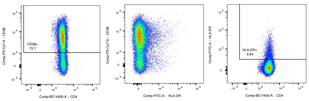
D CD4 gating for HLA-DR and CD38
