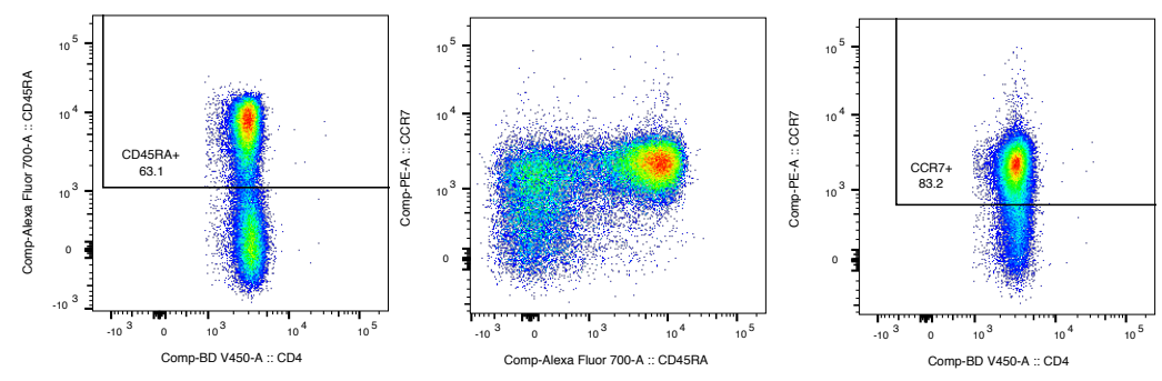
E Boolean gating
