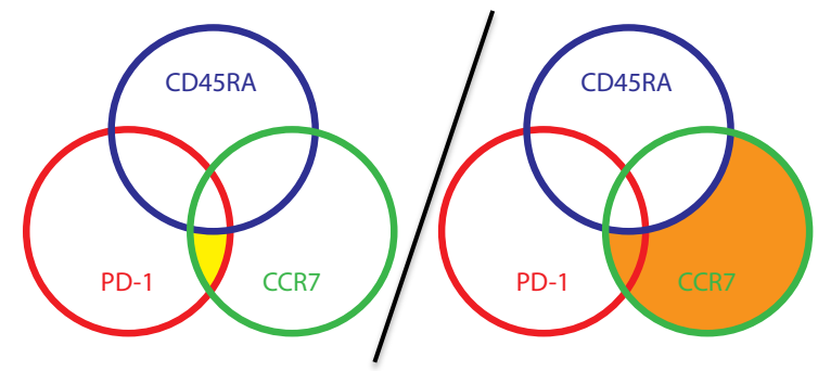
E Boolean gating
