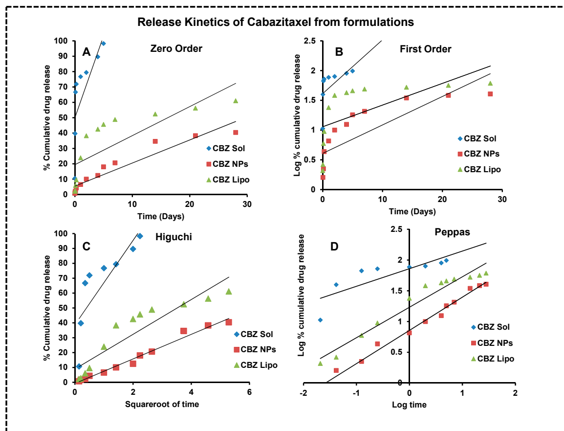
Figure S1. Cabazitaxel release kinetics from different formulations of CBZ Sol (cabazitaxel micellar solution), CBZ NPs (cabazitaxel nanoparticles), and CBZ Lipo (cabazitaxel liposomes): (A) zero-order model, (B) first-order model, (C) Higuchi model, and (D) Peppas model.
