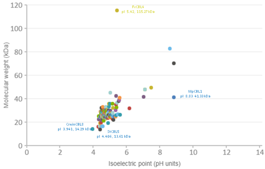
Figure S3. Molecular weight and isoelectric point of CBL Proteins
