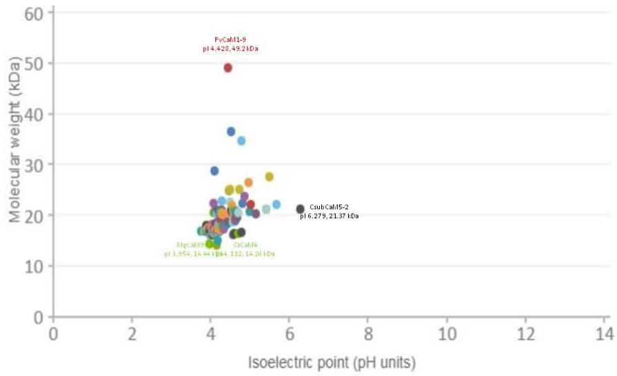
Figure S1. Molecular weight and isoelectric point of CaM Proteins.
