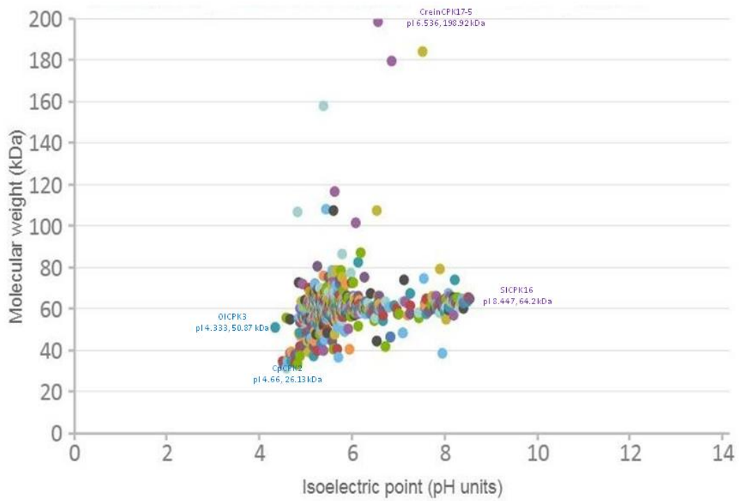
Figure S4. Molecular weight and isoelectric point of CPK Proteins
