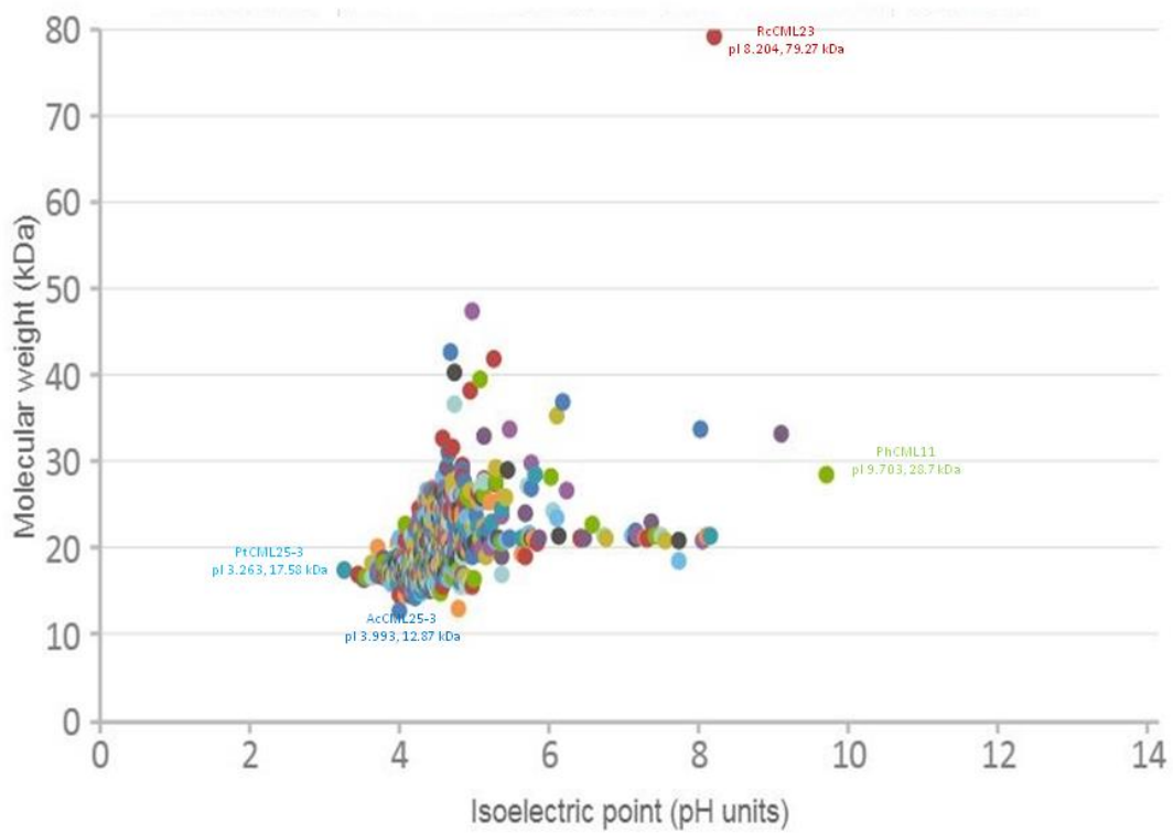
Figure S2. Molecular weight and isoelectric point of CML Proteins
