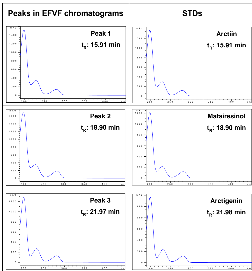
Supplementary Figure 1. Comparison of DAD spectra between major peaks of EFVF and their STDs.
