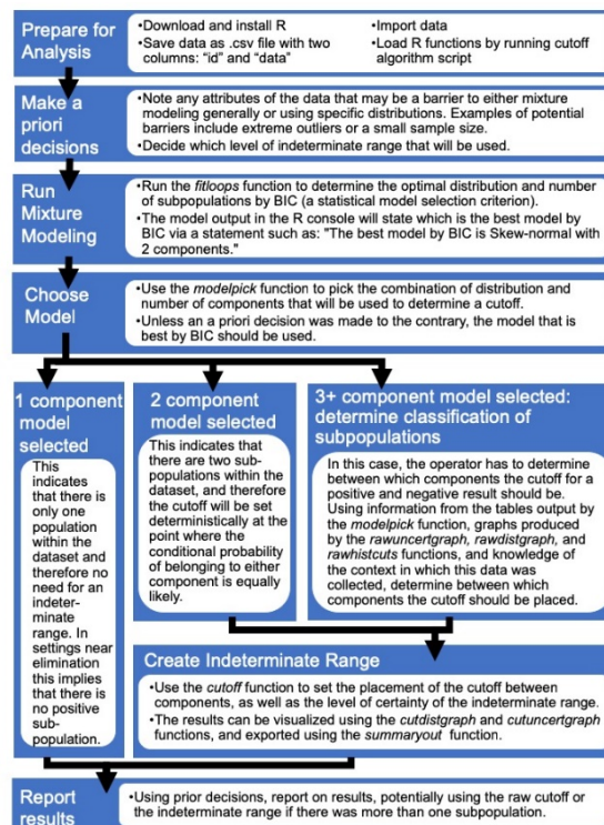
Figure S1. Step-by step guide to mixture modelling algorithms.
