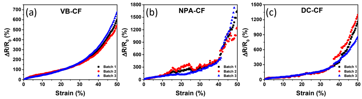
Figure S2. Relative resistance variation ( \Delta R/R_0 ) under tensile loading for textile composites from different batches.
