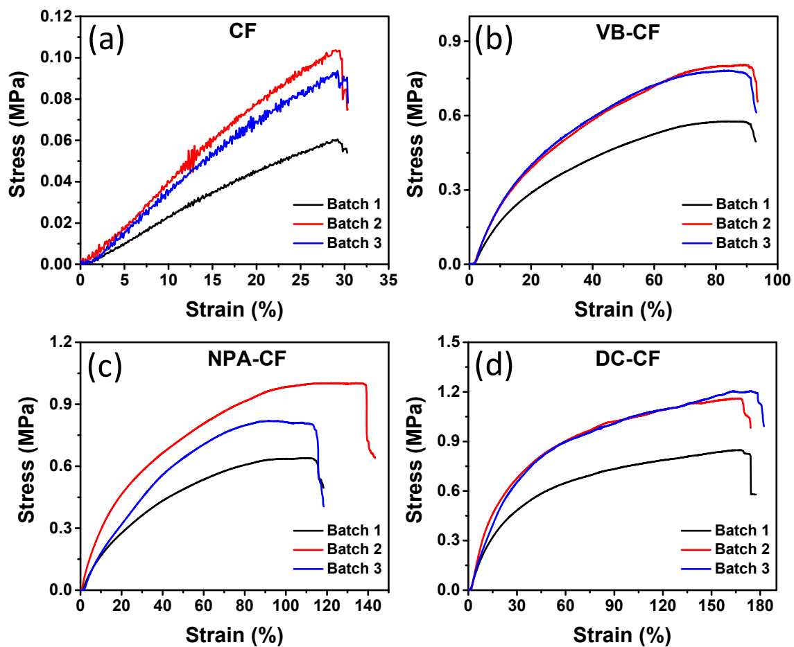
Figure S1. Curves of stress versus strain corresponding to the fabric samples from different batches.
