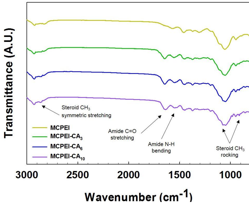
Figure 2. FT-IR spectra of MC-PEI and MCPEI-CAs.
