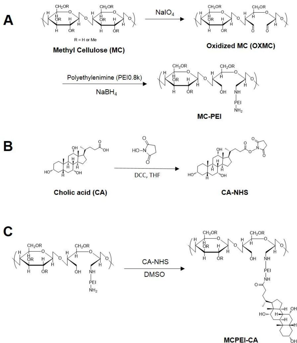
Figure 1. Synthesis scheme of MCPEI-CAs.
