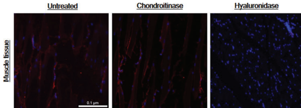
Supplementary Figure S1. Chondroitinase does not target hyaluronan in murine muscle tissue. Left TA muscles of C57Bl6 mice were dissected and immediately transferred into 4% paraformaldehyde, and 9 μm sections were incubated with either 2.5 IU/mL Cho ABC or 150 IU/mL hyaluronidase (3 h at 37°C) or were left untreated. Hyaluronan was detected using biotinylated HABP and streptavidin, with Alexa Fluor ® 555 secondary antibody (red). Nuclei were stained with DAPI (blue).
