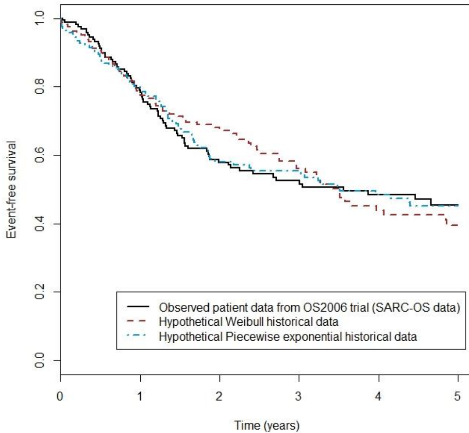
Figure A3: Historical datasets considered in the simulation study
