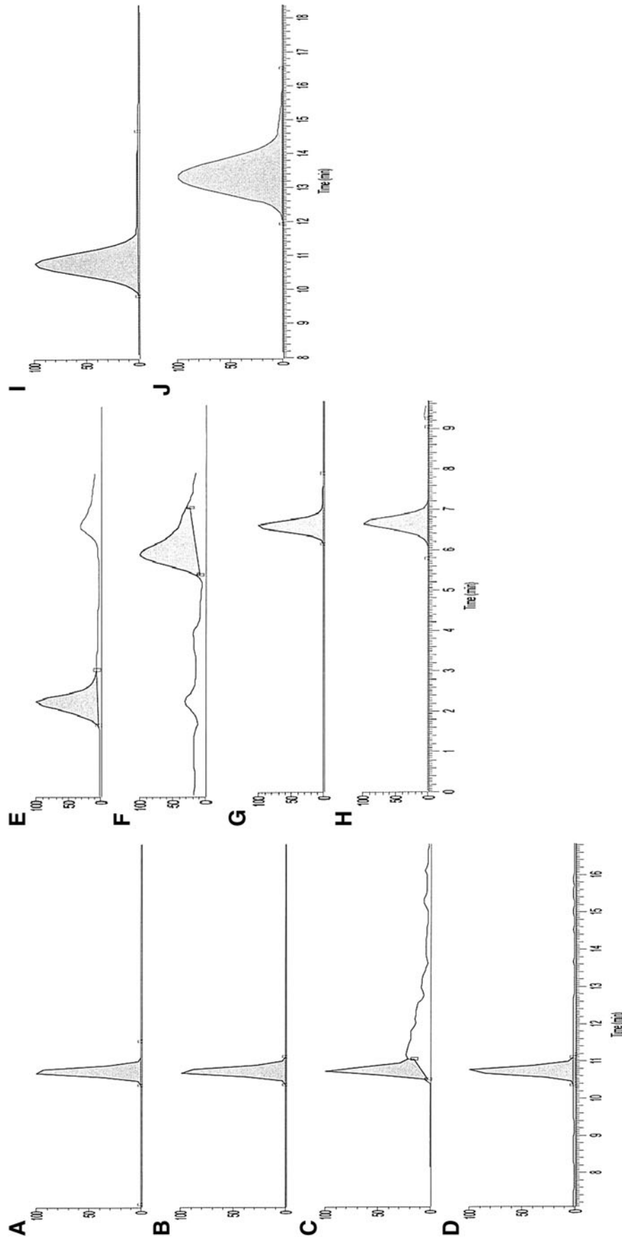
SUPPLEMENTARY FIG. S1. Chromatograms of metabolites of standards sample. (A) NAD + ; (B) NADH; (C) ADPR; (D) NAMN; (E) NAM; (F) NA; (G) NMN; (H) NAAD; (I) NADP + ; (J) NADPH.
