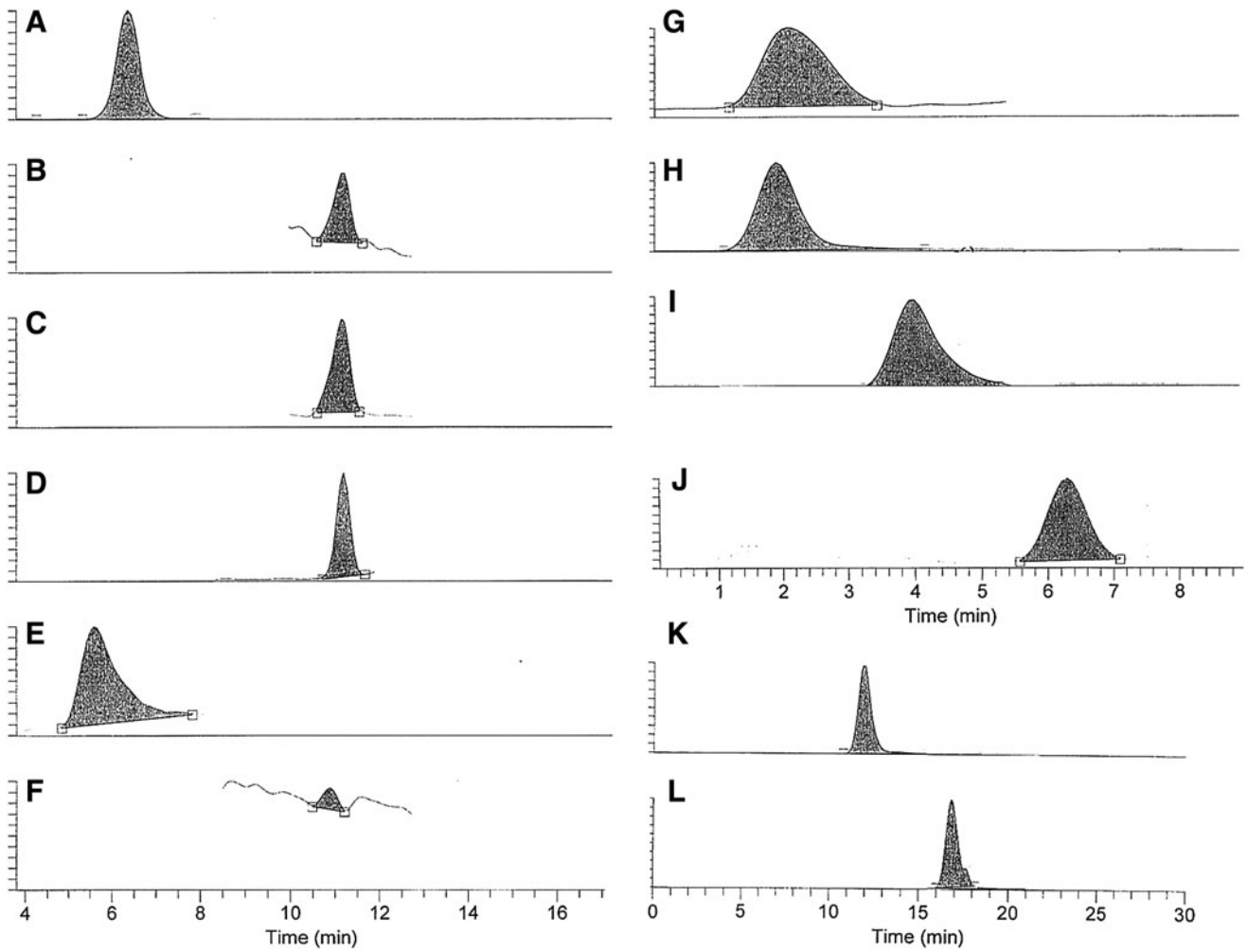
SUPPLEMENTARY FIG. S2. Chromatograms of metabolites in sample. (A) NAD + ; (B) NAAD; (C) NADH; (D) ADPR; (E) NA; (F) NAMN; (G) NAM; (H) d4-NAM; (I) MeNAM; (J) NMN; (K) NADP + ; (L) NADPH.
